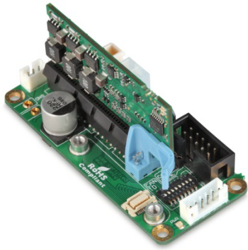
EPOS2 Module Motherboard with attached EPOS2 Module 36/2
