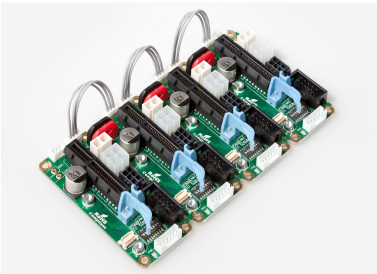
EPOS2 Module Motherboard for four axes
